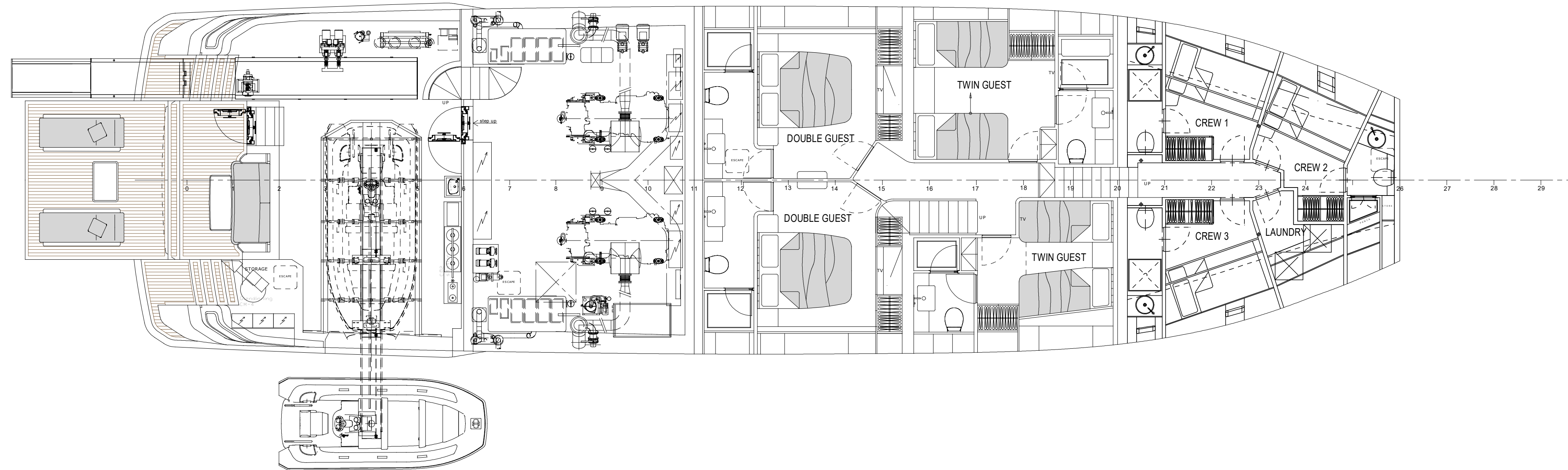
LOWER DECK
